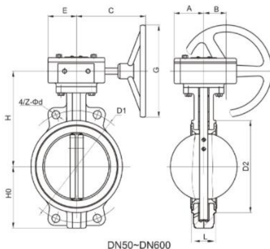
Type2- D371X-10/16C DN50~DN1200 2"~48" Class150 Worm Gear Operated Wafer Concentric Soft Seal Butterfly Valve
